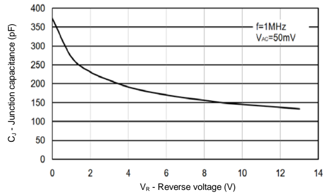
Capacitance vs. Reverse voltage
